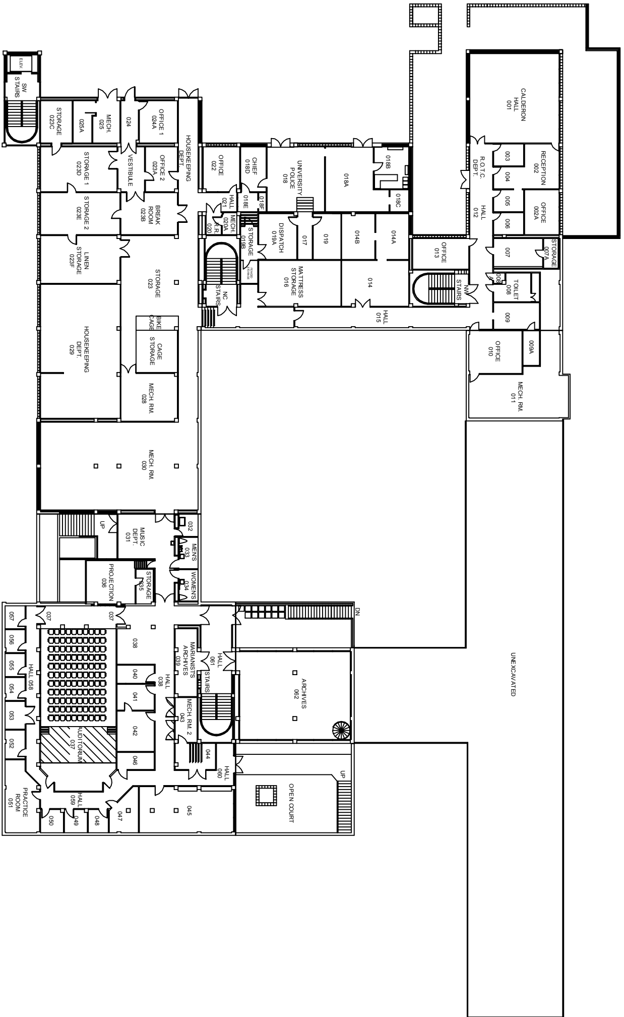
TREADAWAY HALL BASEMENT FLOOR SCALE: NTS
